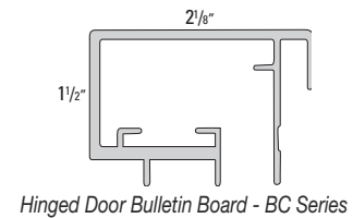
Hinged Door Bulletin Board - BC Series
