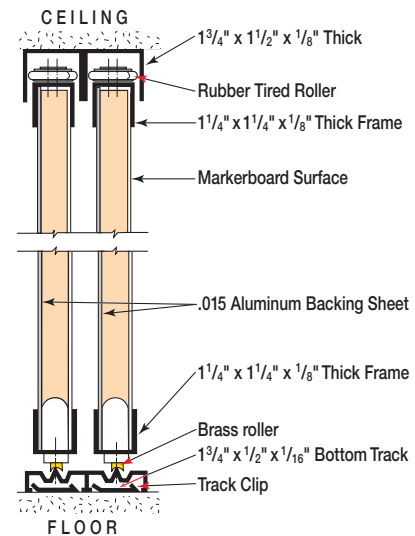
2-Track Unit illustrated (tracks sold separately)
