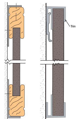
Wood oak frame detail
