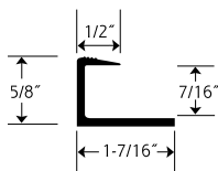
Ramp Frame
